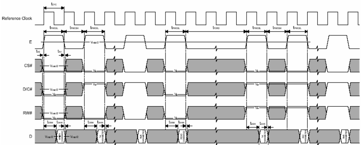
Figure 13-2: 6800 Mode Timing Diagram (Use E as Clock)
