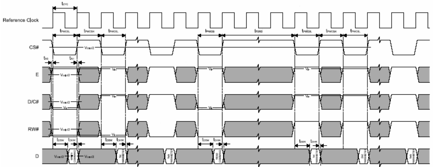
Figure 13-1: 6800 Mode Timing Diagram (Use CS# as Clock)
